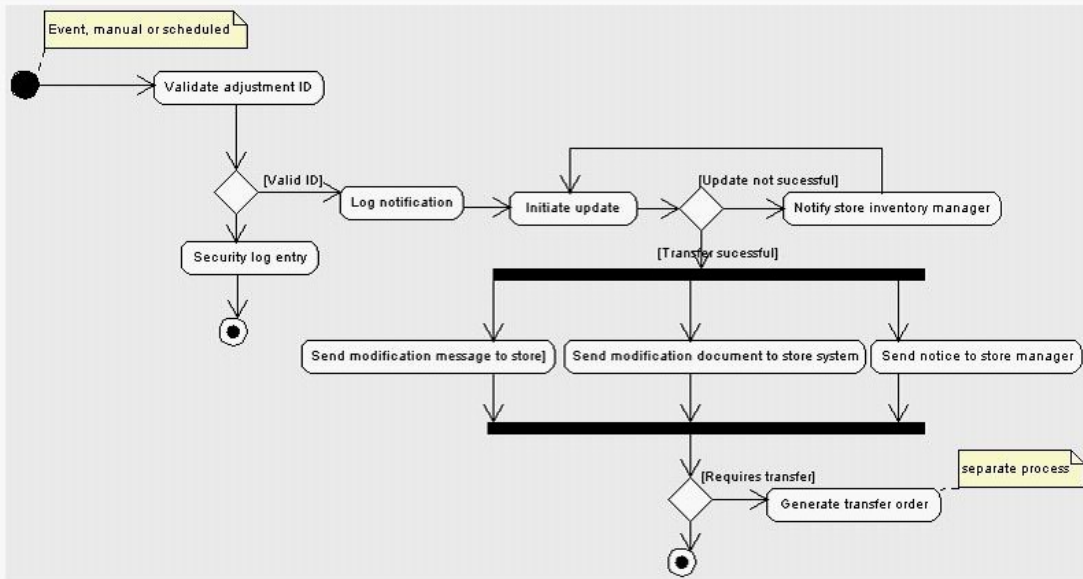
Figure 3.0.2 Adjust Inventory
